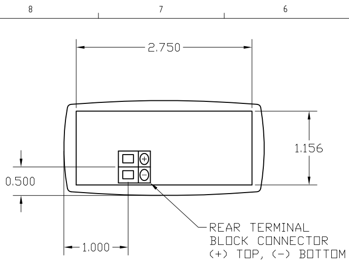
REAR
