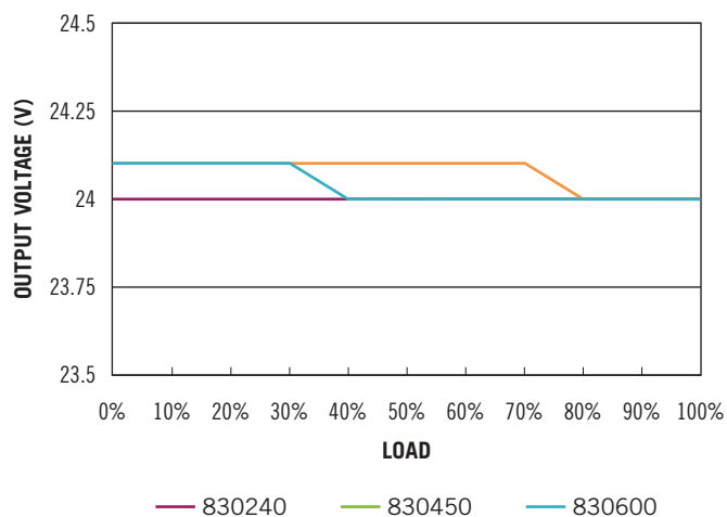
OUTPUT VOLTAGE VS LOAD (2)
