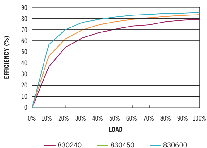
EFFICIENCY VS LOAD (2)
